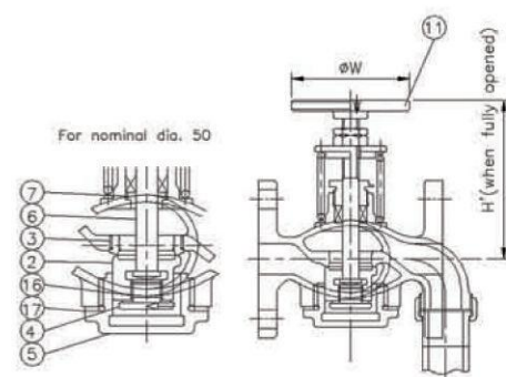
PUSH TYPE
