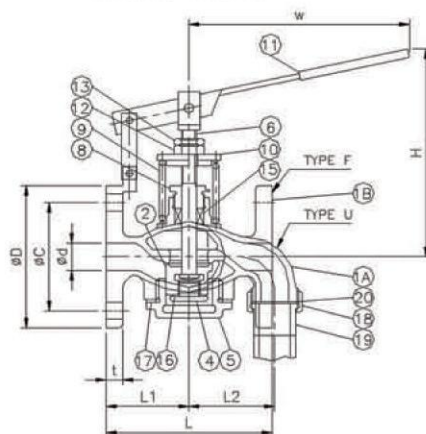
LEVER TYPE
